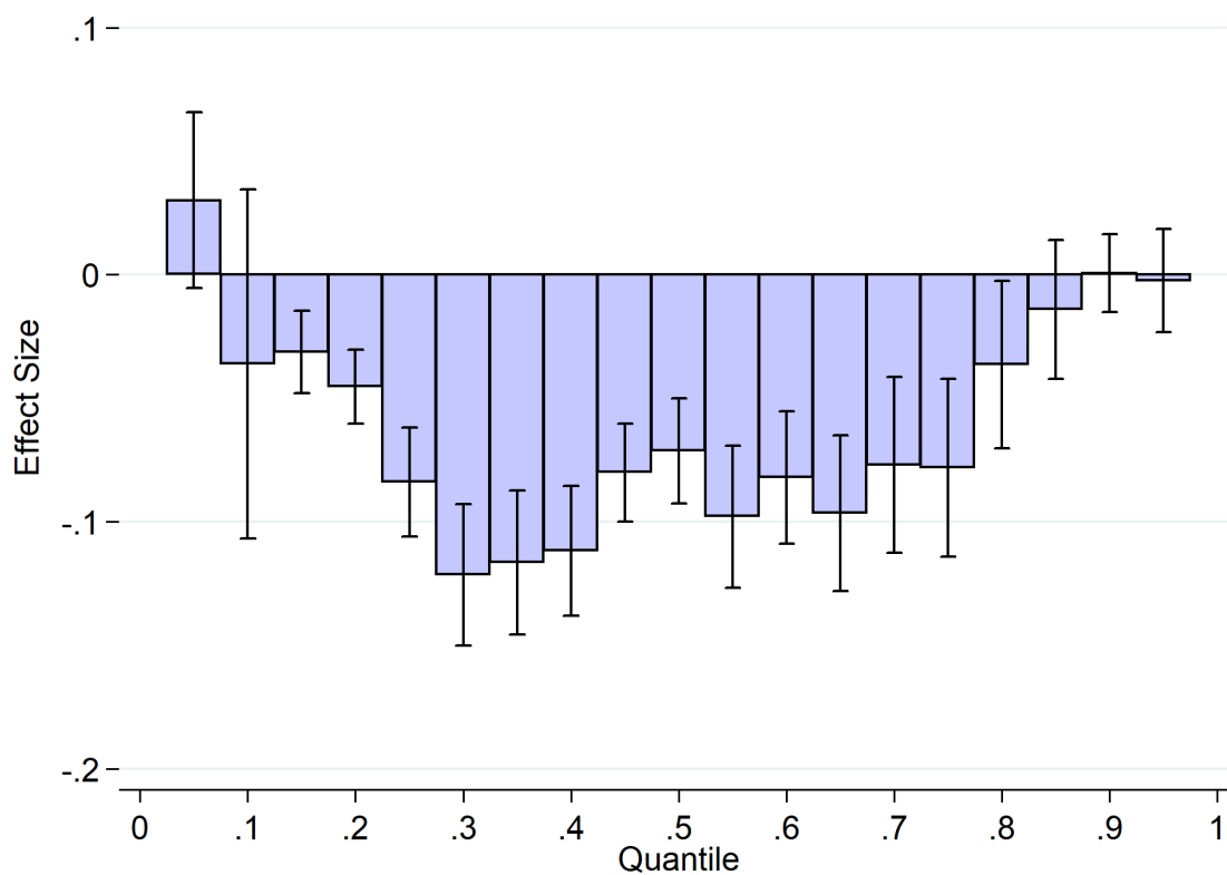
Figure 6: Quantile Effects on \text{asinh}(\text{Total Property Value})
